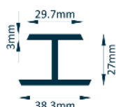
H Joint
