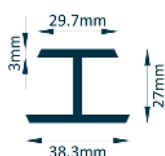
H Joint
