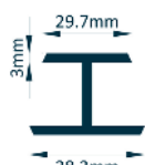
H Joint
